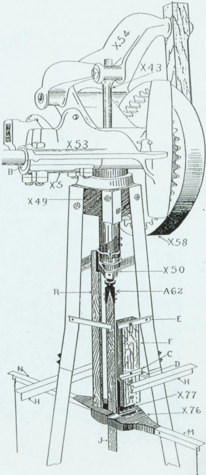
Illustration showing main gearing and governing lever attachment for 8 Whizz
